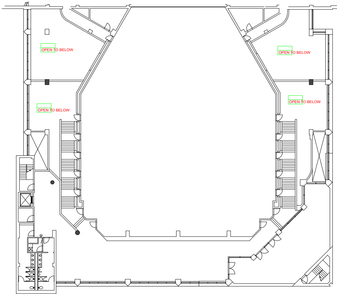
3 A2 3rd Floor Lobby, Grand Tier III Scale: 1/32" = 1'-0"
